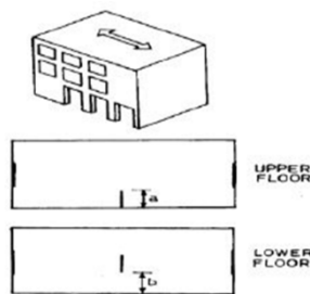
Fig 04 In-Plane Discontinuity in Vertical Elements Resisting Lateral Force
