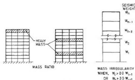
Fig 2 Mass Irregularity
